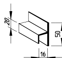
Top Cap Profile
